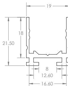
PZM-NFV-CHAN-4 Dimensions
