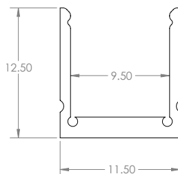
PZM-NFM-CHAN-4 Dimensions
