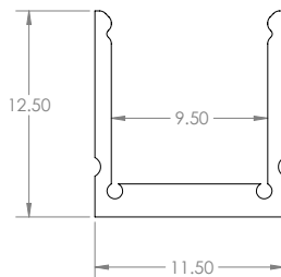
PZM-NFM-CHAN-4 Dimensions
